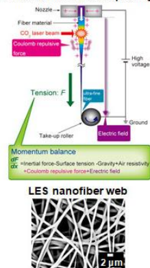
Laser-heated melt electrospinning (LES)
